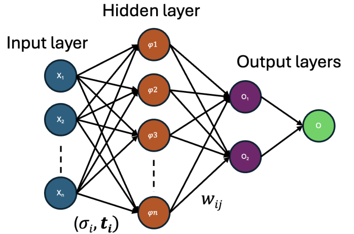
Figure 3: Architecture of the RBF network. The input layer feeds into a hidden layer of radial units, each centered at \mathbf{t}_i with width \sigma_i . The output layer combines the gaussian responses through learned weights w_{ij} , followed by a winner-takes-all decision stage to determine the predicted class.
