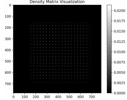
Figure 9: Gram matrix encoding \rho of the digit 1 image
